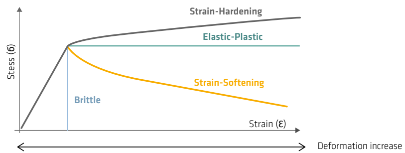
Figure 6.2.1.1: Illustration of strain-softening versus strain hardening
