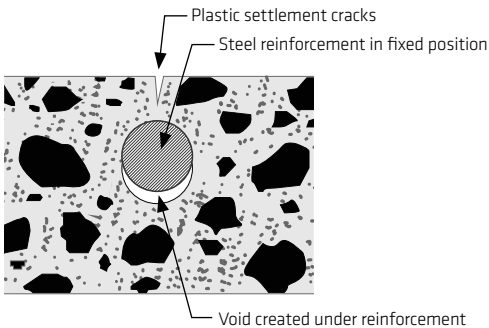
Figure 5.2.1.2: Plastic settlement under a reinforcing bar
