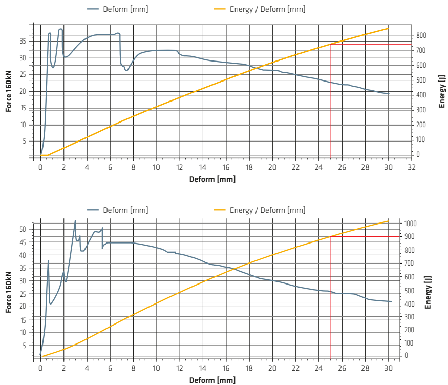
Figures 8.2.1.1: Examples of load/deflection diagrams to determine energy absorption
