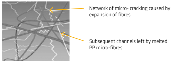
Figure 5.2.3.1: Micro-cracking Network
