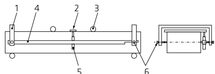
Arrangement of the yoke for measuring bending-deflection
