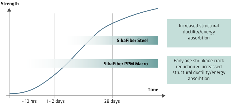
Figure 5.5.1: Macro-fibres influences
