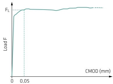
Strain hardening
