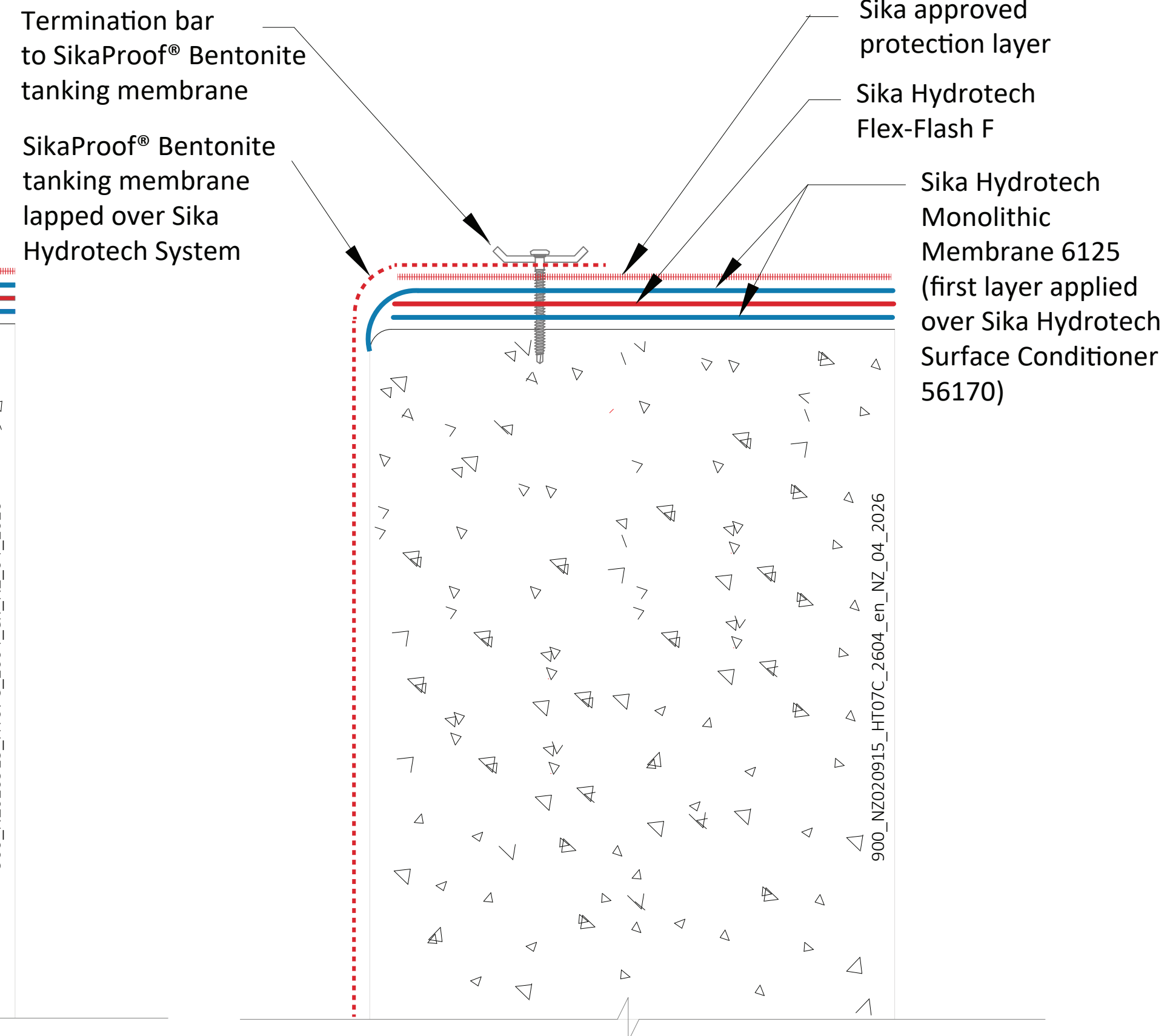
Horizontal Lap Under SikaProof Bentonite Tanking
