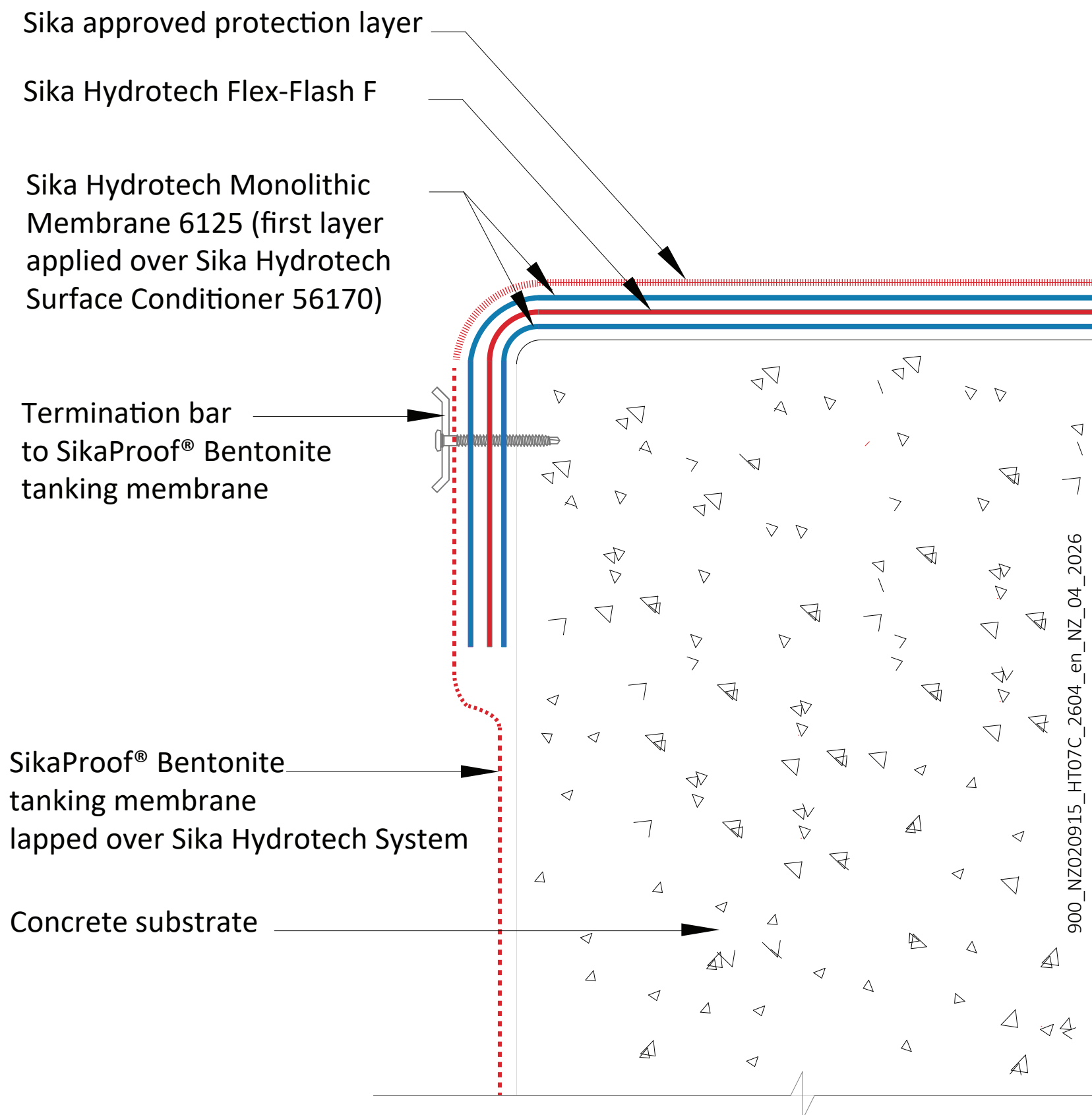
Vertical Lap Under SikaProof Bentonite Tanking
