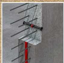
Construction joint
