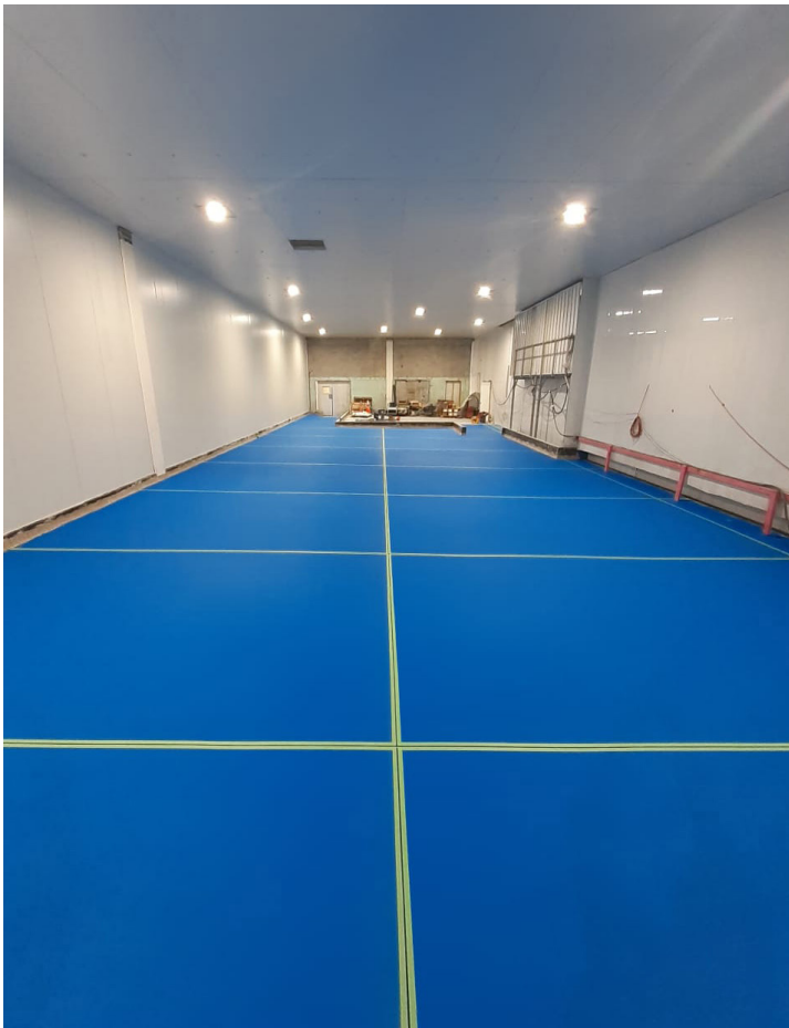
The Sikafloor PurCem products are installed and ready for joint sealant, to complete a hygienic floor system
