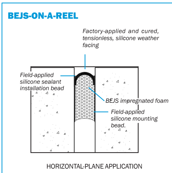
BEJS-ON-A-REEL provides a 12-ft (3.6 m) length on a single reel.
