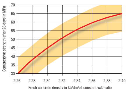
Fig. 6.12.1: Influence of density on compressive strength
