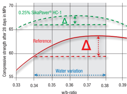
Fig. 6.12.2: Influence of w/b-ratio on compressive strength
