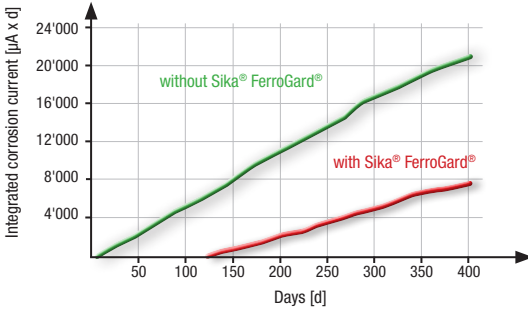
Fig. 8.2.3: The Sika Research Department in Zurich tested the anticorrosive effect of Sika® FerroGard® on cracked concrete beams.
