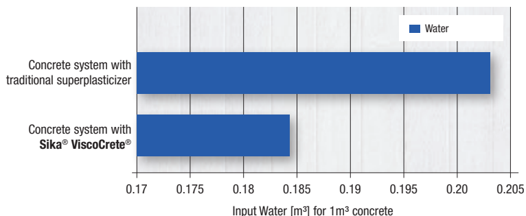
Fig. 2.3.1: Input Net Freshwater with and without Sika® ViscoCrete®
