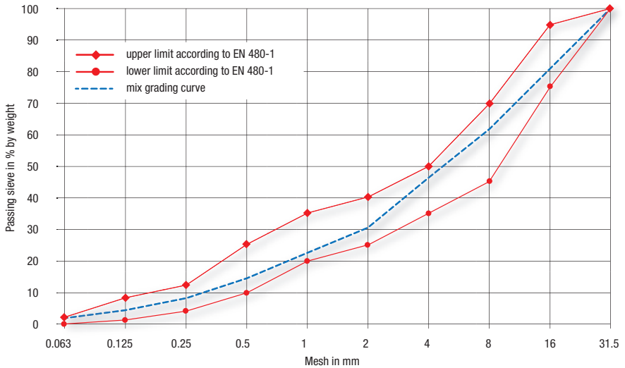
Fig. 4.1.1: Particle size distribution (grading curve range according to EN 480-1)
