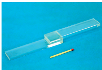
Fig. 3 Test sample. Lap shear test with PMMA substrate bonded with different adhesives. One sample has been screwed
