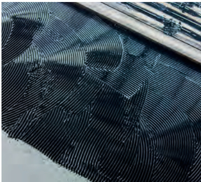
Fig. 12 Sikaflex®-298 applied with a comb spreader
